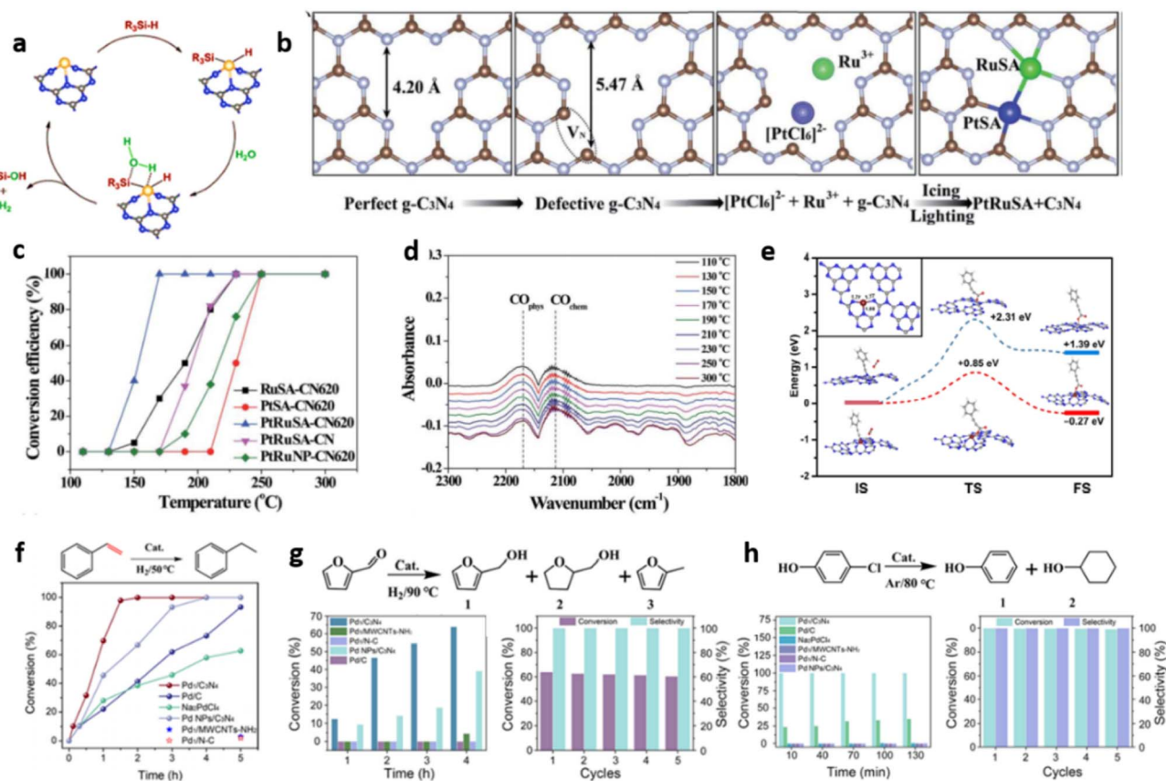
Fig. 25 (a) The plausible mechanism of \text{Au}_1/\text{mpg-C}_3\text{N}_4 catalysed water-based silane oxidation. Reproduced with permission from ref. 26. Copyright 2017 John Wiley and Sons. (b) Scheme for the synthesis of PtRuSA-CN620 by the photoreduction method, (c) CO conversion over synthesised catalysts at CO concentration of 1 vol%, (d) CO oxidation monitored by in situ infrared spectra using PtRuSA-CN620. Reproduced from ref. 8. Under the terms of Creative Commons License, published 2019 Royal Society of Chemistry. (e) Reaction profile for \text{CO}_2 insertion over Cu-CN-8.0 & CN catalysts (inset: the optimised structure of Cu-CN-8.0). Reproduced with permission from ref. 112. Copyright 2020 American Chemical Society. Reaction scheme and catalytic performance of \text{Pd}_1/\text{C}_3\text{N}_4 for (f) hydrogenation of styrene, (g) hydrogenation of furfural (h) hydrodechlorination of 4-chlorophenol. Reproduced with permission from ref. 113. Copyright 2020 American Chemical Society.
