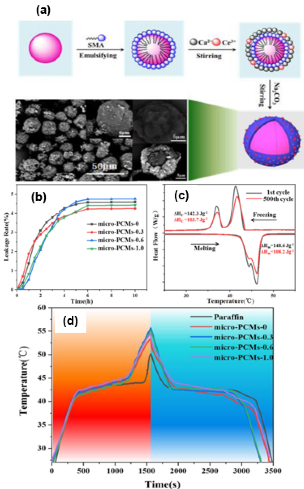
Fig. 19 (a) Schematic of synthesis for paraffin microcapsules composed of Ce^{3+} doped calcium carbonate with SEM images; (b) Leakage rate of paraffin microcapsules; (c) DSC curves of PCM microcapsules containing 0.6 wt% Ce^{3+} with respect to calcium carbonate; (d) paraffin and paraffin microcapsules' temperature–time curves during the release processes (blue) and storage (red). 177 Reproduced with permission from ref. 177 Copyright 2019 ACS.
