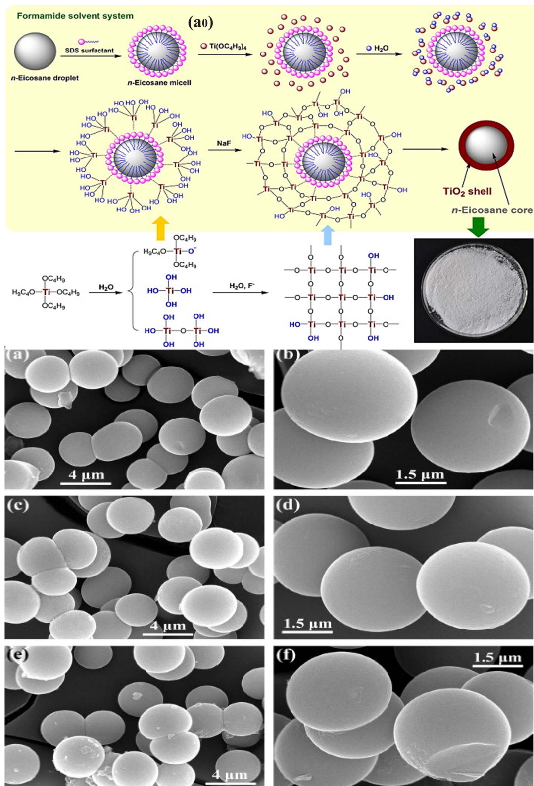
Fig. 15 (a0) Schematic illustration of the fabrication of the n\text{-eicosane} microcapsule \text{TiO}_2 shell, SEM images of the n\text{-eicosane} microcapsule (a and b) produced with a weight ratio of 60/40 n\text{-eicosane/TBT} , (c and d) produced with a weight ratio of 50/50 n\text{-eicosane/TBT} , and (e and f) produced with a weight ratio of 40/60 n\text{-eicosane/TBT} . 129 Reproduced with permission from ref. 129 Copyright 2015 Elsevier.
