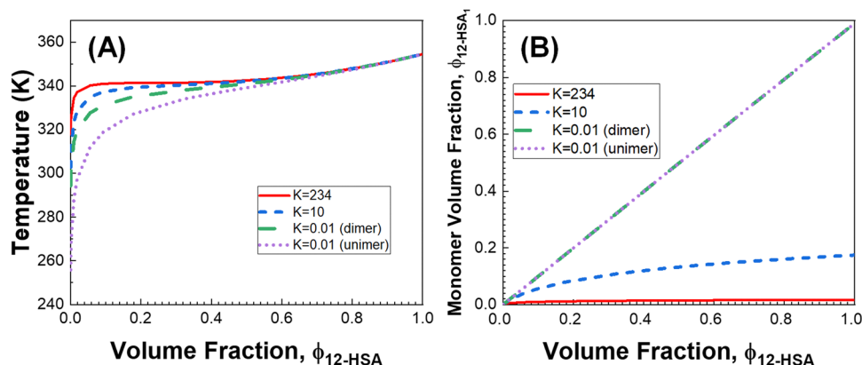
Fig. 6 (A) Predicted liquidus lines for 12-HSA in octane at K = 234 , 10, and 0.01 for 12-HSA dimers and K = 0.01 for a 12-HSA unimer using eqn (13) with B = 0.4 , \Delta H_{f,12-HSA}^\circ = 100\,900\text{ J mol}^{-1} (dimer) and 50\,450\text{ J mol}^{-1} (unimer), V_{12-HSA} = 625\text{ cm}^3\text{ mol}^{-1} (dimer) and 312.5\text{ cm}^3\text{ mol}^{-1} (unimer), V_s = 163.6\text{ cm}^3\text{ mol}^{-1} , V_r = 163.6\text{ cm}^3\text{ mol}^{-1} . (B) Monomer volume fraction ( \phi_{12-HSA_1} ) vs. 12-HSA volume fraction for the predicted liquidus lines shown in (A).
