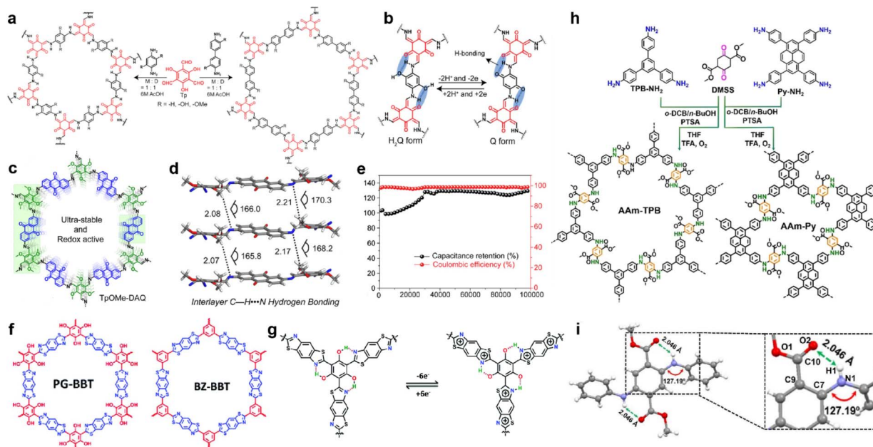
Fig. 8 (a) Synthesis of pPa- R_2 [TpPa-1, TpPa-(OH) _2 , and TpPa-(OMe) _2 ] and TpBD- R_2 [TpBD, TpBD-(OH) _2 , and TpBD-(OMe) _2 ] where R = H, OH, and OMe. (b) Proposed H-bonding stabilizing both the hydroquinone (H _2 Q) and benzoquinone (Q). Reprinted from ref. 85. Copyright 2017, American Chemical Society. (c) Structure of TpOMe-DAQ. (d) Interlayer C—H \cdots N H-bonding in TpOMe-DAQ. (e) Cycling stability performance (10 mA cm ^{-2} ) of the TpOMe-DAQ electrode. Reprinted from ref. 89. Copyright 2018, American Chemical Society. (f) Structure of PG-BBT and BZ-BBT. (g) Intramolecular hydrogen bonds and charge–discharge process of the benzobisthiazole unit. Reprinted from ref. 71. Copyright 2020, Royal Society of Chemistry. (h) Synthetic routes for arylamine-linked COFs. (i) Intralayer N—H \cdots O hydrogen bonding in a model compound of arylamine-linked COF. Reprinted from ref. 93. Copyright 2021, Wiley-VCH Verlag GmbH.
