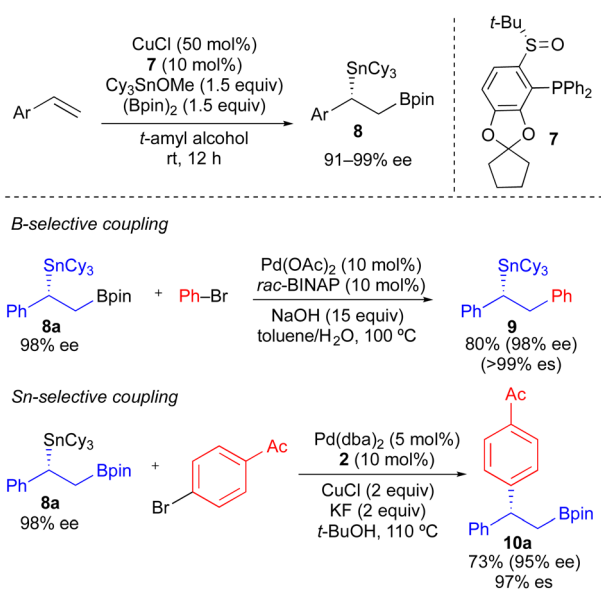
Scheme 5 Formation of enantioenriched \alpha -aryl- \beta -borylstannanes via asymmetric Cu-catalyzed borylstannylation of styrenes, and their use in B-selective and Sn-selective cross-coupling reactions.
