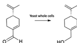
Scheme 1 Reduction of ( S )-perillaldehyde into ( S )-perillyl-alcohol.
