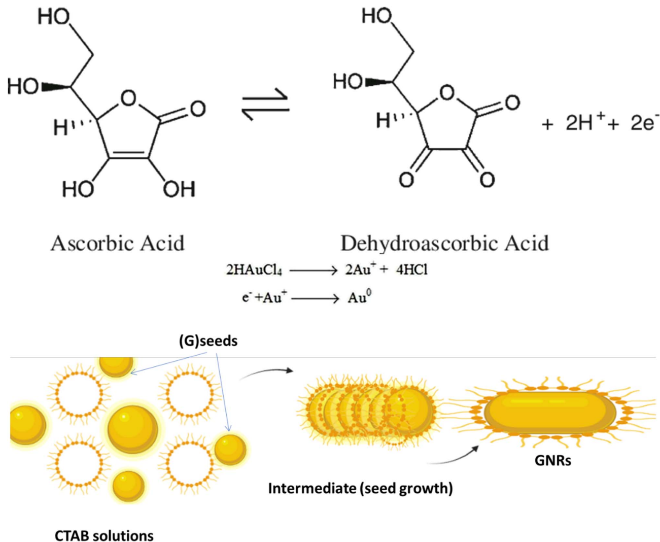
Fig. 1 Illustrates the reduction mechanism of (G) ions (Au 3+ ) to elemental (G) (Au 0 ) by (AA) and the role of CTAB in controlling the anisotropic (GNR) growth. CTAB molecules on the seed surface control the deposition and arrangement of (G) atoms during the reduction process, producing rod-shaped nanoparticles. By regulating the concentration and interaction of CTAB and the reaction conditions, it becomes possible to control the size and aspect ratio of the (GNR) synthesized using Murphy's (GNR) synthesis technique. The interplay among (AA), CTAB, and (G) ions enables the controlled growth of anisotropic (GNPs).
