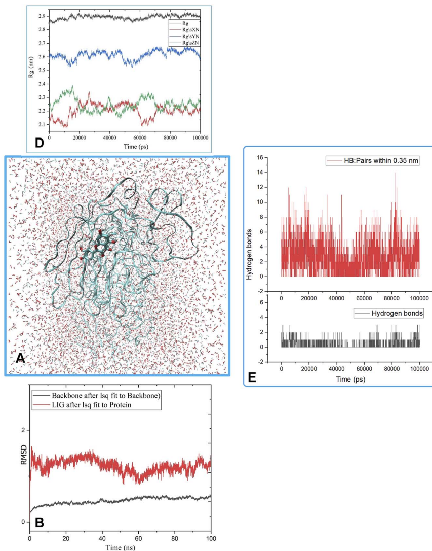
Fig. 11 (A) MD simulation analysis of the best pose 120/400 to receptor, 3TOP: A chain, (B) the root means square deviation (RMSD) of (5a) and protein backbone 3TOP calculated using 100 ns MD simulation, (C) root mean square fluctuations (RMSF), (D) radius of gyration ( R_g ) plot, (E) the number of hydrogen bonds.
