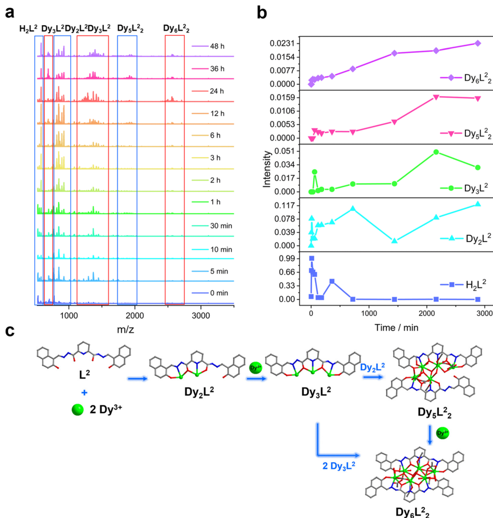
Fig. 6 (a) Time-dependent HRESI-MS tracking of the HNP- \text{Dy}_6 formation process, (b) HRESI-MS spectra intensity–time profiles of the species, and (c) schematic of the possible assembly mechanism of HNP- \text{Dy}_6 .
