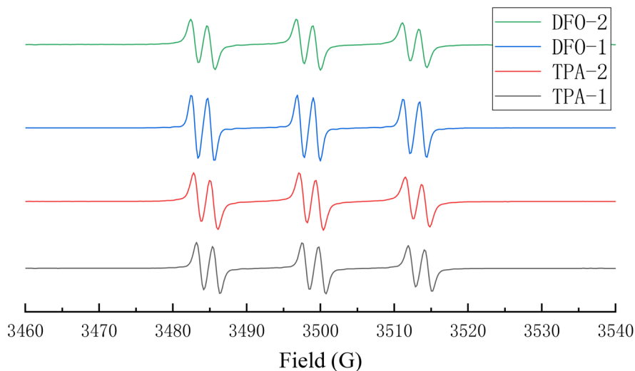
Fig. 7 Electron spin resonance spin trapping spectra of the chalcones/lod systems.
