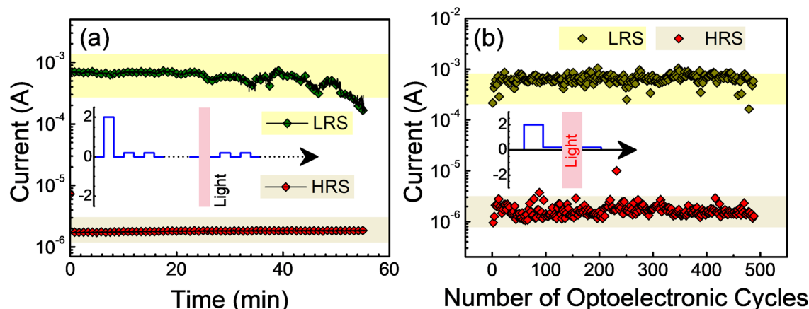
Fig. 4 The current output of a device based on Ag 2 BiI 5 under a +0.2 V voltage pulse (a) after an LRS or an HRS was induced by a +2.0 V pulse and an illumination, respectively and (b) when the two states were imposed by a combination of +2.0 V pulse and illumination and then flipped in sequence to study the cyclic reproducibility; the states were probed with a read voltage of +0.2 V after each input. The sequence of the write voltage pulse, the illumination, and the read voltage are shown in the respective insets. While the 1 sun illumination was shined for 1 s, the width of the write and read voltage pulses was 100 ms.
