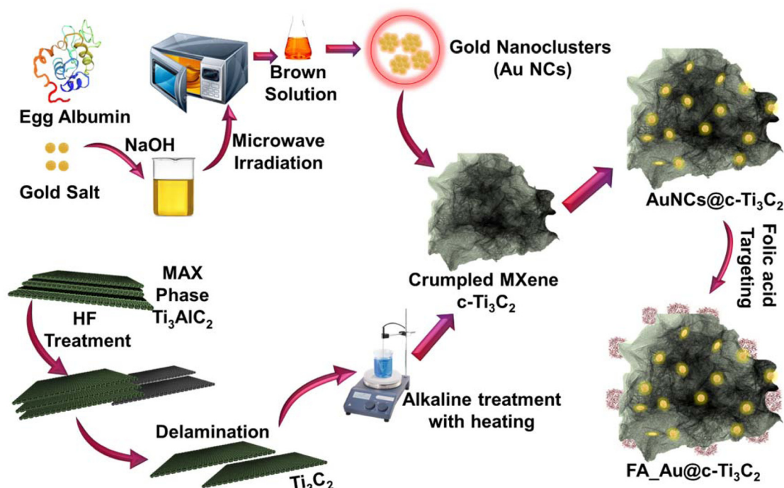
Scheme 1 Synthesis procedure of the folic acid conjugated MXene gold composite (FA_Au@c-Ti 3 C 2 ).
