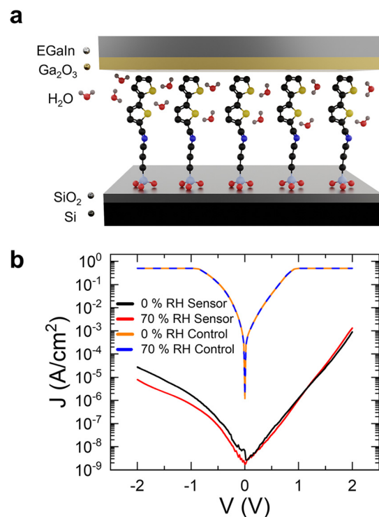
Fig. 2 (a) Molecular rectifier device structure with BT-TESP-MA SAM molecules sandwiched between the \text{Si}/\text{SiO}_2 and EGaIn electrodes interacting with water molecules. (b) The current density versus voltage curves for the molecular humidity sensor based on the BT-TESP-MA monolayer for low and high humidity. The substrate response (control) is included for reference.
