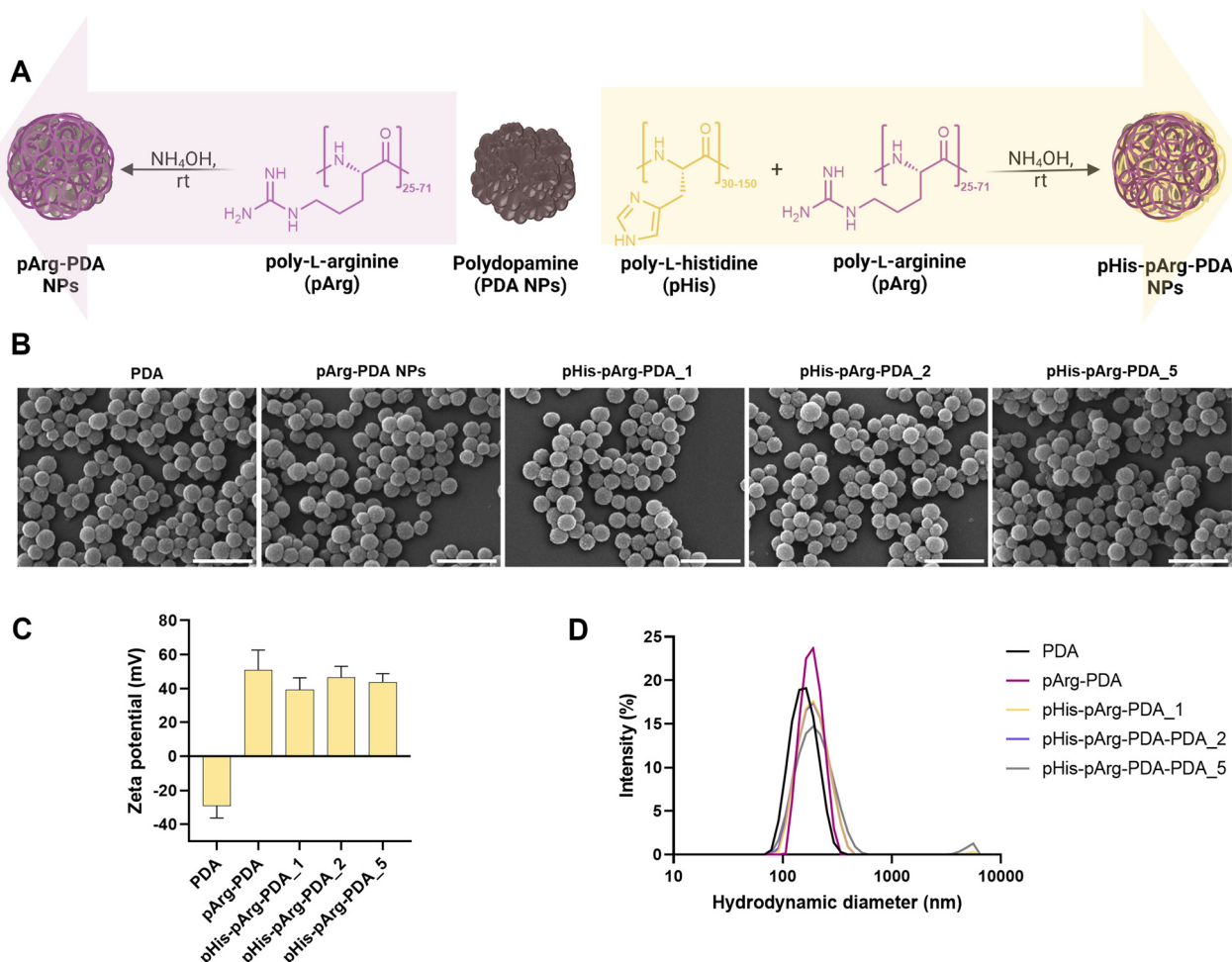
Fig. 1 Synthesis and characterisation of pArg-PDA and pHis-pArg-PDA NPs. (A) Scheme showing the functionalisation of PDA NPs with pArg and pHis-pArg-PDA NPs. (B) SEM micrographs of PDA, pArg-PDA, pHis-pArg-PDA 1 , pHis-pArg-PDA 2 and pHis-pArg-PDA 5 NPs. The NPs were dispersed on a glass slide and coated with 10 nm sputtered Pt. Scale bar is 500 \mu m. (C) Zeta ( \zeta )-potential and (D) hydrodynamic size of PDA, pArg-PDA, pHis-pArg-PDA 1 , pHis-pArg-PDA 2 and pHis-pArg-PDA 5 NPs obtained from dynamic light scattering measurements (DLS) in water.
