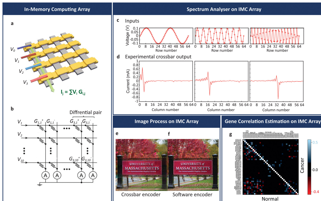
Fig. 3 In-memory computing using an RRAM array. (a) Schematic of an RRAM array. The output current is the sum of several channels of voltage times the corresponding node conductance. (b) Schematic of the array with differential pair, where the differential output makes the array more robust. (c)–(f) Spectrum analyser using an RRAM array based on differential VMM, where with the input voltage signal (c) times the pre-programmed array weights, the array can output current at respective column expressing the frequency component of the input signals (d). With the functional hardware spectrum analyser, image encoding (two-dimensional discrete cosine transform, 2D-DCT) using an RRAM array (e) in comparison to the software encoder (f). (g) Gene correlation estimation on the IMC array. Partial correlation computed of 40 genes for cancer and normal tissues (only displayed correlation greater than 0.13 for visualization reason). Credits: (a) is reproduced with permission from ref. 74, copyright Zidan et al. 2018 Springer Nature; (b) is reproduced with permission from ref. 69, copyright Prezioso et al. 2015 Springer Nature Limited; (c)–(f) are reproduced with permission from ref. 73, copyright Li et al. 2018 Springer Nature; (g) is reproduced with permission from ref. 77, copyright Gallo et al. 2018 Springer Nature.
