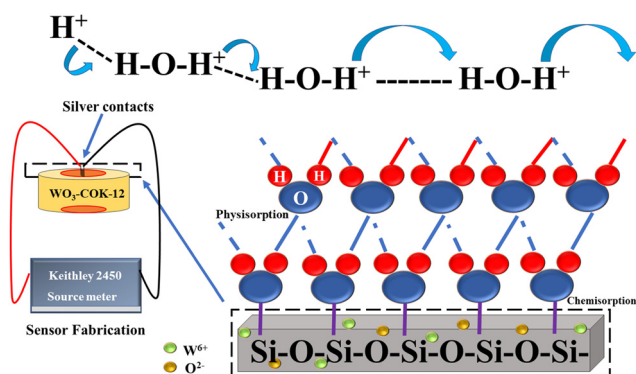
Fig. 12 Illustration of the Grotthuss chain mechanism in WO 3 /COK-12 showcasing the proton-conducting process within the sensing material.
