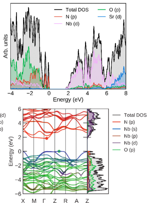
Fig. 12 (left) Total and projected densities of states and (right) band structure for SrNbO 2 N, calculated at the HSE06 level.
