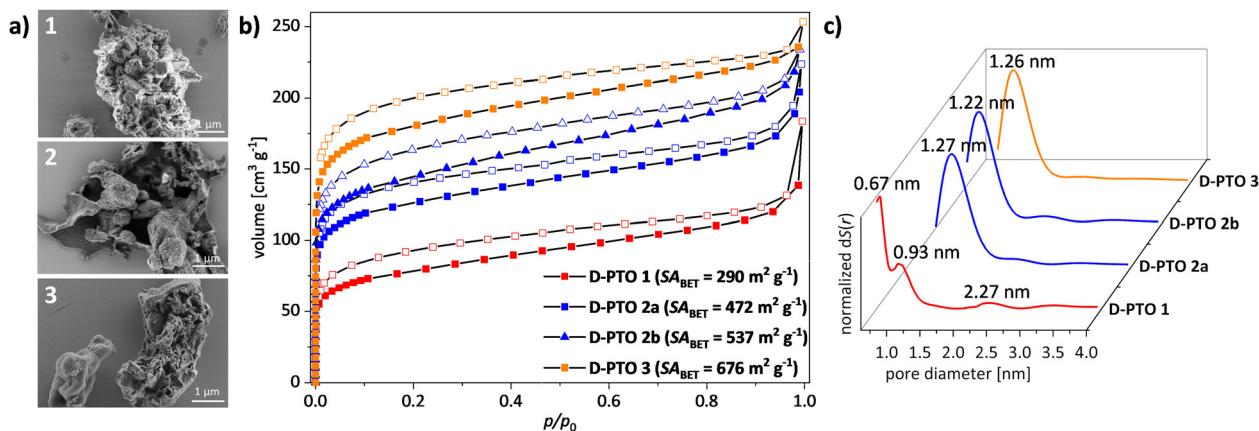
Fig. 5 (a) SEM images of D-PTO-1 , -2a , and -3 (from top to bottom). (b) BET gas sorption isotherms ( \text{N}_2 , 77 K, vector dosing) after activation at 120 °C for 12 h. (c) pore size distribution (QSDFT, Kernel: \text{N}_2 on carbon at 77 K, sphere/cylindrical pore).
