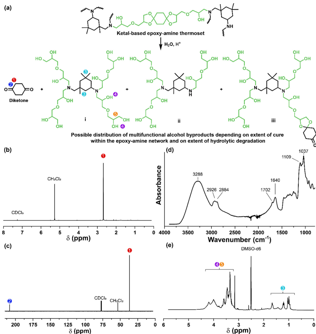
Fig. 7 (a) Degradation of thermoset 3P under acidic aqueous conditions to yield 1,4-cyclohexanedione and a mixture of multifunctional alcohol structures. (b) ^1H NMR of 1,4-cyclohexanedione obtained from the organic phase. (c) ^{13}C NMR of 1,4-cyclohexanedione obtained from the organic phase. (d) FTIR of the multifunctional alcohol mixture obtained after lyophilization of the neutralized aqueous phase. (e) ^1H NMR of the multifunctional alcohol mixture; due to the inability to separate the products, only general NMR peak assignments are made.
