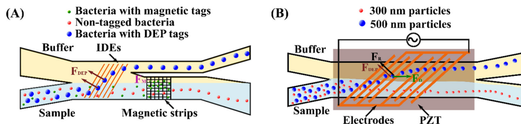
Fig. 5 Hybrid microfluidic techniques for sorting submicron and nanoparticles. (A) Sorting multiple bacterial targets by serially combining DEP and MP in an integrated DEP-MP cell sorter. 251 (B) A vDLD system for sorting sub-micrometre particles by coupling acoustic and DEP forces. 252
