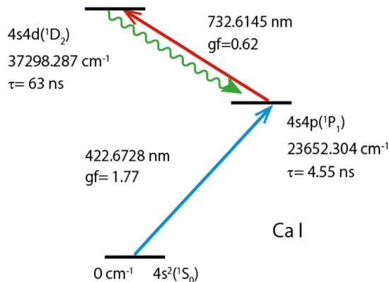
Fig. 2 Two-color two-step resonance excitation and fluorescence observation scheme of atomic Ca. Lifetimes ( \tau ) of ^1P_1 and ^1D_2 levels were cited from ref. 43,44, oscillator strengths (gf) of the first and second transitions from ref. 45,46, level-energies, and transition wavelengths (in air) and configurations from ref. 47,48.
