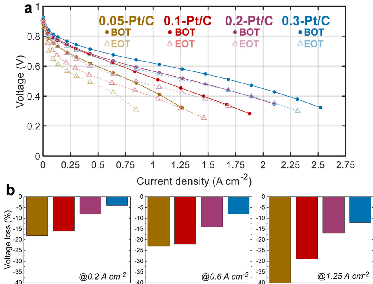
Fig. 1 (a) Polarization curves for the MEAs comprising 0.05-Pt/C, 0.1-Pt/C, 0.2-Pt/C and 0.3-Pt/C cathode CLs at BOT and EOT; (b) voltage losses of selected points at low ( 0.2\ A\ cm^{-2} ), medium ( 0.6\ A\ cm^{-2} ) and high ( 1.25\ A\ cm^{-2} ) current densities.
