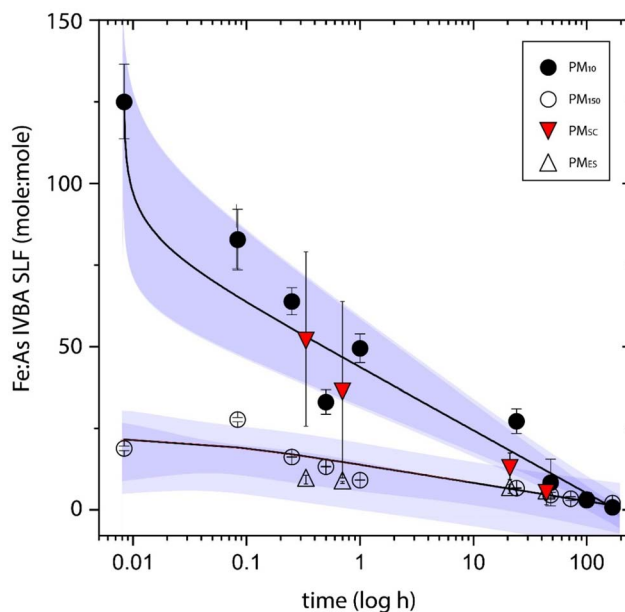
Fig. 4 Mole ratio of released iron and arsenic in SLF. Solid circles are PM_{10} , open circles are PM_{150} , closed downward red triangles are PM_{5C} , open triangles PM_{ES} , lines represent the best fit ( y = a - b \cdot \ln(x + c) ) to the data, PM_{10} R^2 = 0.946, PM_{150} R^2 = 0.829, fits to SC and ES not shown. Dark shaded bands represent the 95% confidence interval, light shading represents the 95% prediction band.
