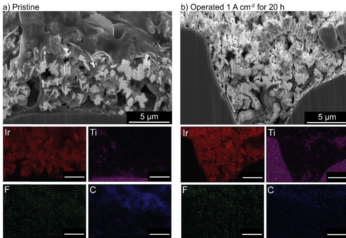
Fig. 5 Cross-sectional imaging and EDX of an \text{IrO}_x /20% TP-85 anode PTE. (a) Before and (b) after 20 h operation at 1 \text{ A cm}^{-2} . All scale bars are 5 \mu\text{m} . No ionomer is observed in the catalyst layer after operation.
