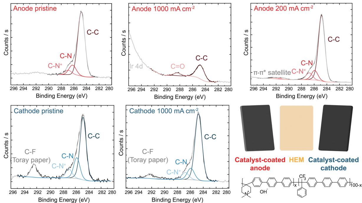
Fig. 4 XPS analysis of \text{IrO}_x /20% TP-85 anode and Pt-black/10% TP-85 cathode. C 1s spectra of (a) anode and (b) cathode PTE. Inset shows the chemical structure of the TP-85 ionomer. Ionomer degradation is only observed on the anode PTE operating at high current.
