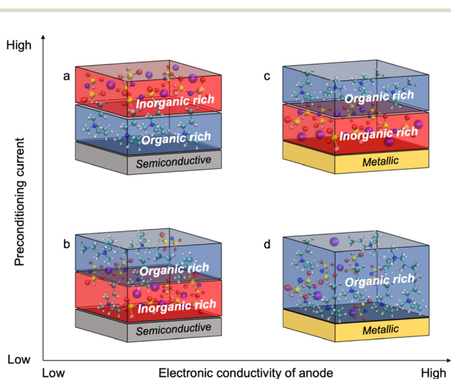
Fig. 4 Schematic relationships between the SEI composition, applied preconditioning current, and dielectric nature of the anode material. The semiconductive electrode cycled with 50 mol% NaFSI in [C 3 mpyr][FSI] at (a) high and (b) low rates. The metallic electrode cycled with 50 mol% NaFSI in [C 3 mpyr][FSI] at (c) high and (d) low rates. The colour codes of atoms are as follows: nitrogen (blue), sulphur (yellow), sodium (purple), carbon (aqua blue), hydrogen (white), oxygen (red), and fluorine (pink).
