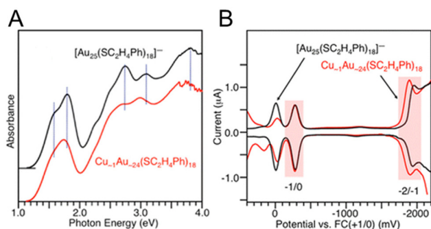
Fig. 10 (A) Optical absorption spectra of \text{Cu}_{1-1}\text{Au}_{24}(\text{PET})_{18} and [\text{Au}_{25}(\text{PET})_{18}]^- . The dotted lines indicate the main peak positions in the absorption spectrum of [\text{Au}_{25}(\text{PET})_{18}]^- . (B) DPV curves of \text{Cu}_{1-1}\text{Au}_{24}(\text{PET})_{18} and [\text{Au}_{25}(\text{PET})_{18}]^- . The red shaded regions indicate the peaks derived from the redox potentials of -2/-1 and -1/0 . Reproduced with permission from ref. 111. Copyright 2012, American Chemical Society.
