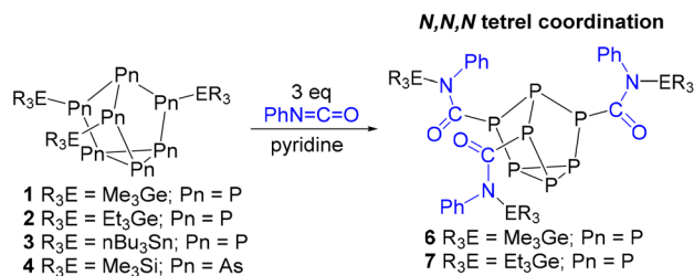
Scheme 2 Reaction of neutral (R_3E)_3Pn_7 clusters with phenyl isocyanate.
