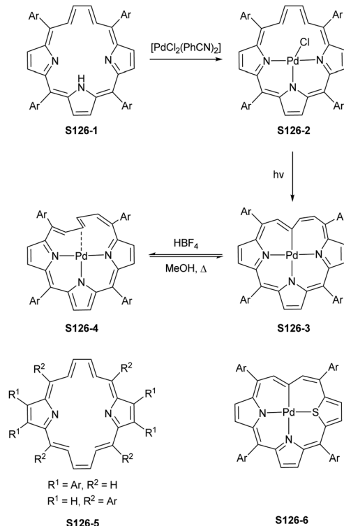
Scheme 126 Vacata- ( S126-1 ), divacata- ( S126-5 ), and allyliporphyrin ( S126-6 ) frameworks.
