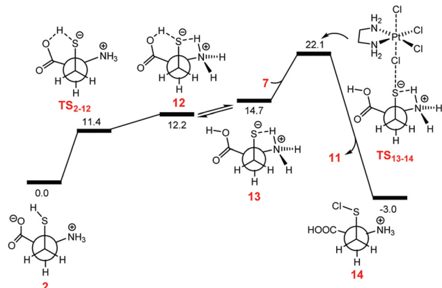
Fig. 2 Free energy profile describing the inner-sphere ligand-bridged reduction of the [\text{Pt}(\text{en})\text{Cl}_4] complex by Cys. Reproduced from ref. 40 with permission. Copyright 2018 by The Royal Society of Chemistry.
