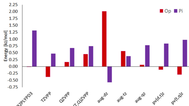
Fig. 2 Electronic energy differences for conformations in the methanol–furan complex with OH-bonded top Ot reference at different levels of theory. The left most left bar contains the only DFT results at B2PLYPD3/6-311++g(d,p)B3PLYPD3/6-311++g(d,p) level, all other energies refer to DLPNO-CCSD(T) energies. The capitalized basis sets are Ahlrichs def2-(T or Q)ZVPP and its extrapolation; the lower case basis sets are aug-cc-pv(d, t, or q)z basis sets and two extrapolations of them.
