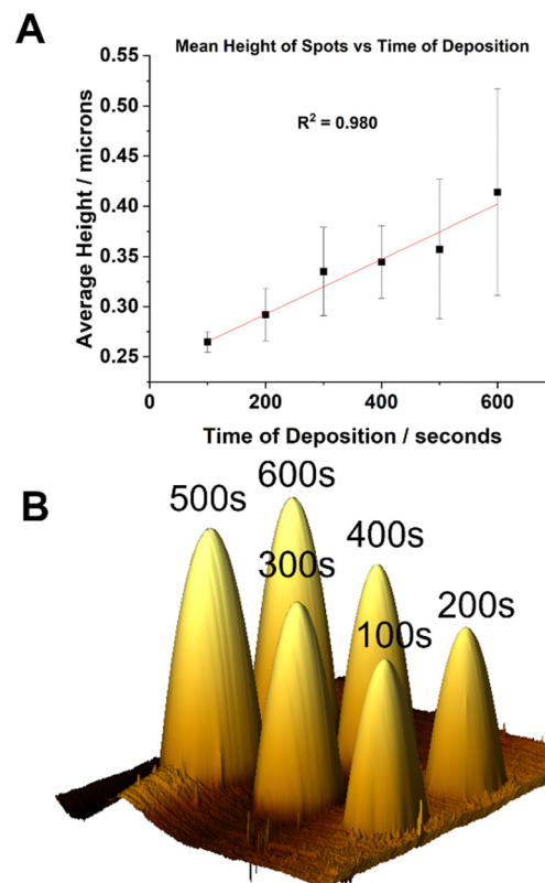
Fig. 4 Si-eATRP of Am at a SAM-functionalised gold electrode using [\text{Am}] = 10\text{ wt\%} and [\text{Cu}^{\text{II}}]/[\text{TPMA}] = 6.9\text{ mM} ; (A) feature height as function of reaction time; (B) 3D representation of the AFM image of features deposited at E_{\text{app}} = -0.15 V at increasing reaction times (100–600 s).
