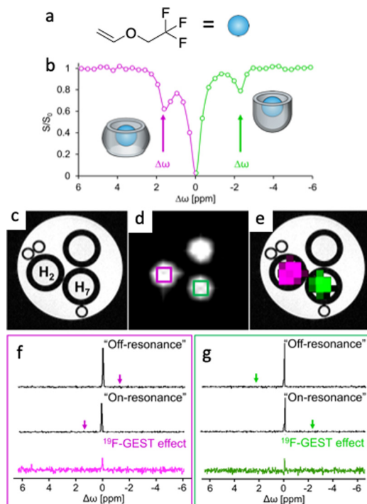
Fig. 9 Diamagnetic GEST: (a) the chemical structure of the fluorinated anesthetic fluorexene used as an inhalable ^{19}\text{F} -guest. (b) ^{19}\text{F} -NMR z-spectrum obtained from an aqueous solution containing a mixture of cucurbit[7]uril (H2) and dimeric octa acid (H7). The sample contained 5 mM fluorexene and 10 \mu\text{M} of each host. (c) ^1\text{H} -MRI, (d) ^{19}\text{F} -MRI, and (e) ^{19}\text{F} -GEST map of a three-tube phantom containing 5 mM fluorexene and 5 \mu\text{M} of either cucurbit[7]uril (H2) or octa acid (H7). A tube with 5 mM fluorexene only was used as a control. (f and g) Localized ^{19}\text{F} -GEST spectroscopy data of two voxels acquired from the tubes containing (f) H2:fluorexene (magenta) or (g) H7:fluorexene (green). The ^{19}\text{F} -GEST spectra represent the subtraction of the ^{19}\text{F} -NMR spectra obtained when the saturation pulse was applied "on-resonance" from the ^{19}\text{F} -NMR spectra obtained when the saturation pulse was applied "off-resonance." Data were acquired with a 9.4 T MRI scanner with B_1 = 2.5 \mu\text{T}/2 \text{ s} . For fluorexene@H2, "on-resonance" was \Delta\omega = +1.6 \text{ ppm} and "off-resonance" was \Delta\omega = -1.6 \text{ ppm} . For fluorexene@H7, "on-resonance" was \Delta\omega = -2.2 \text{ ppm} and "off-resonance" was \Delta\omega = +2.2 \text{ ppm} . Modified with permission from ref. 83.
