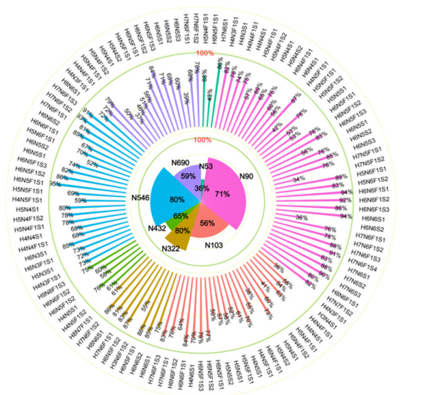
Fig. 4 The distribution of \alpha -2,3-sialylation on N -glycopeptides and specific glycosites of hACE2. The contents of \alpha -2,3-linked sialic acid isomer of glycans on specific N -glycosites are labeled in the outer circle, corresponding to the glycan compositions. The overall proportions of \alpha -2,3-sialylation presented on specific N -glycosites are illustrated in the inner circle. N53, N90, N103, N322, N432, N546 and N690 are colored green, pink, carmine, toast tan, grass green, blue, and purple, respectively.
