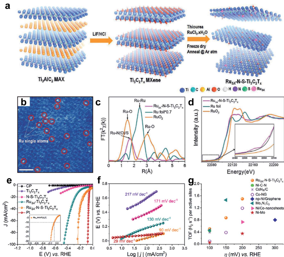
Fig. 11 (a) Schematic illustration of the RuSA-N-S-Ti 3 C 2 T x synthetic route. (b) HAADF-STEM image of RuSA-N-S-Ti 3 C 2 T x . Scale bar, 2 nm. (c) FT-EXAFS spectra and (d) the normalized Ru K-edge XANES spectra of Ru foil, RuO 2 and RuSA-N-S-Ti 3 C 2 T x . (e) HER polarization curves of bare carbon paper (CP), Ti 3 C 2 T x , N-S-Ti 3 C 2 T x , RuSA-Ti 3 C 2 T x , Pt and RuSA-N-S-Ti 3 C 2 T x in 0.5 M H 2 SO 4 ; inset: the magnified view of RuSA-N-S-Ti 3 C 2 T x . (f) Tafel plots corresponding to e; (g) TOF of the RuSA-N-S-Ti 3 C 2 T x catalyst compared with previously reported metal-based HER electrocatalysts. Reprinted with permission from ref. 75. Copyright 2019 John Wiley and Sons.
