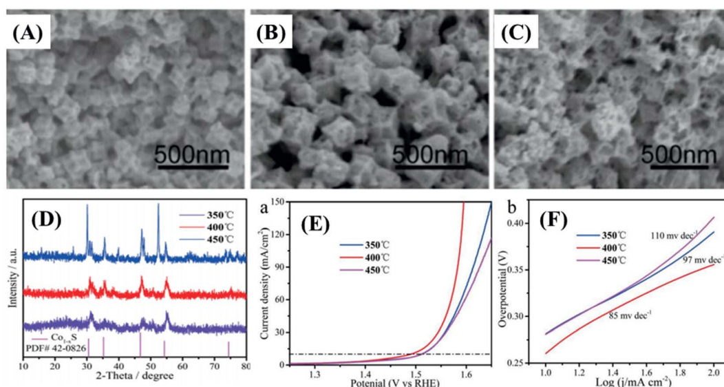
Fig. 19 SEM images of an amorphous \text{CoS}_x@\text{C} sample calcined at (a) 350 °C, (b) 400 °C and (c) 450 °C, and the respective (d) XRD patterns, (e) iR -compensated LSV polarization curves and (f) Tafel plots. Reproduced with permission. 93 Copyright© 2018. Published by Elsevier B.V. on behalf of the Chinese Chemical Society and the Institute of Materia Medica, Chinese Academy of Medical Sciences.
