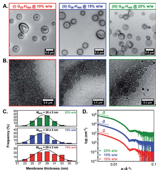
Fig. 1 Characterization of G_{59} - H_{400} diblock copolymer precursor vesicles prepared via RAFT-mediated aqueous PIDA when targeting (i) 10% w/w, (ii) 15% w/w or (iii) 20% w/w solids: (A) representative dry-state TEM images obtained using a 0.75% w/w uranyl formate staining solution; (B) corresponding representative cryo-TEM images; (C) membrane thickness distribution histograms and mean membrane thicknesses, determined by analyzing at least 100 vesicles in each case; (D) SAXS patterns recorded for 1.0% w/w aqueous vesicle dispersions.
