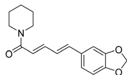
Piperine
