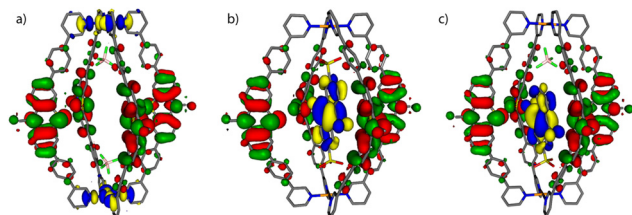
Fig. 4 Frontier molecular orbital visualization of (a) donor-functionalized cage \mathbf{1} (containing two \text{BF}_4^- counter anions), and host-guest assemblies (b) [\mathbf{G1@1}]^{2+} and (c) [\mathbf{G3@1} + \text{BF}_4]^{2+} . The HOMOs are represented in red-green, LUMOs in yellow-blue.
