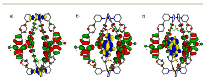
Fig. 4 Frontier molecular orbital visualization of (a) donor-functionalized cage \mathbf{1} (containing two \text{BF}_4^- counter anions), and host-guest assemblies (b) [\mathbf{G1@1}]^{2+} and (c) [\mathbf{G3@1} + \text{BF}_4]^{2+} . The HOMOs are represented in red-green, LUMOs in yellow-blue.
