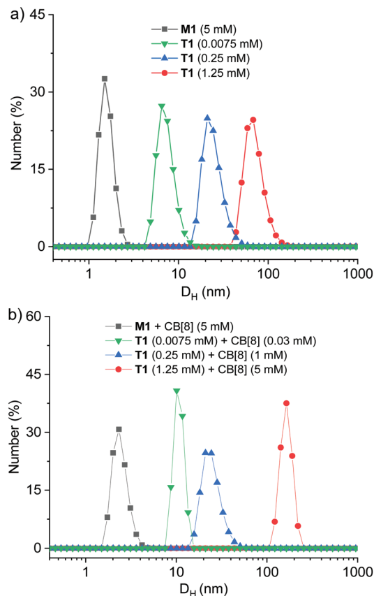
Fig. 4 Dynamic light scattering profile of (a) the solution of M1 and T1 in water and (b) the solution of the mixture of M1 (1 : 1) and T1 (1 : 4) with CB[8] in H 2 O at 25 °C.
