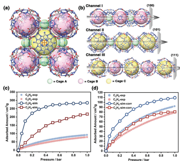
Fig. 1 (a) An orthogonal stacking of the three cages in the crystal structure of JNU-2, where Cage A , B , and C are highlighted in coloured spheres. H atoms are omitted for clarity. Colour representation: gold, Cu; dark blue, Zn; blue, N; grey, C; red, O. (b) Three possible gas diffusion channels in JNU-2. (c) GCMC simulated adsorption isotherms of C_2H_6 and C_2H_4 in reference to the experimental data. (d) The corrected GCMC simulated adsorption isotherms of C_2H_6 and C_2H_4 in reference to the experimental data.
