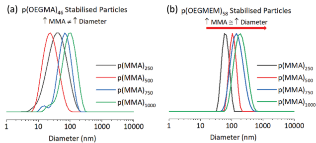
Fig. 3 Comparison of (a) p(\text{OEGMA})_{46} - b - [\text{p}(\text{MMA})_y\text{-st-}p(\text{EGDMA})_x] , and (b) p(\text{OEGMEM})_{58} - b - [\text{p}(\text{MMA})_y\text{-st-}p(\text{EGDMA})_x] particle DLS traces, showing intensity weighted data. The traces highlight the narrower dispersity of the p(\text{OEGMEM})_{58} stabilised particles (b) in comparison to the p(\text{OEGMA})_{46} stabilised particles (a), of which the Z-average diameters and PDIs are shown in Table 1.
