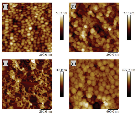
Fig. 4 AFM images: (a) p(\text{OEGMEM})_{58} - b - [\text{p}(\text{MMA})_{430}\text{-}p(\text{EGDMA})_5] , (b) p(\text{OEGMEM})_{58} - b - [\text{p}(\text{MMA})_{620}\text{-}p(\text{EGDMA})_8] , (c) p(\text{OEGMA})_9 - b - [\text{p}(\text{MMA})_{730}\text{-}p(\text{EGDMA})_8] , (d) p(\text{OEGMEM})_{58} - b - [\text{p}(\text{MMA})_{1500}\text{-}p(\text{EGDMA})_{25}] .
