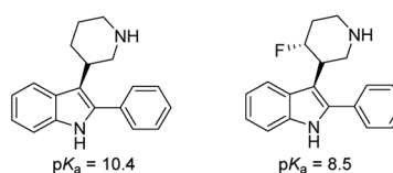
Scheme 56 pK_a value of fluorinated and non-fluorinated piperidines.
