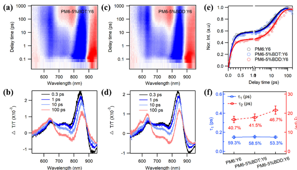
Fig. 5 (a) 2D color plot of fs TA spectra of PM6-5%BDT:Y6 blend films under 750 nm excitation. (b) Representative fs TA spectra of PM6-5%BDT:Y6 at indicated delay times. (c) 2D color plot of the fs TA spectra of PM6-5%BDD:Y6 blend films under 750 nm excitation. (d) Representative fs TA spectra of PM6-5%BDD:Y6 at indicated delay times. (e) Hole transfer kinetics and the fitting results. (f) Comparisons of \tau_1 and \tau_2 of the blends.
