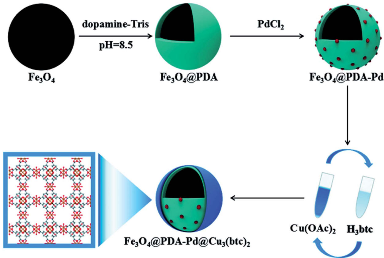
Fig. 9 Schematic of the procedure for the synthesis of the \text{Fe}_3\text{O}_4@PDA-Pd@[Cu_3(BTC)_2] nanocomposite. This figure was adapted with permission from ChemCatChem , 2018, 10, 1446–1454. 77
