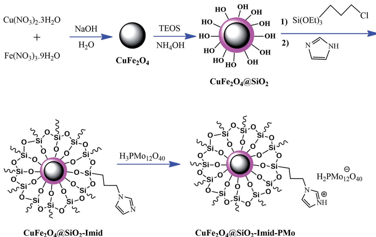
Fig. 13 Synthesis of \text{CuFe}_2\text{O}_4@(\text{SiO})_2\text{-Imid-PMo} catalyst. This figure was adapted with permission from: Quarterly Journal of Iranian Chemical Communication , 2019, 7, 271–282. 99
