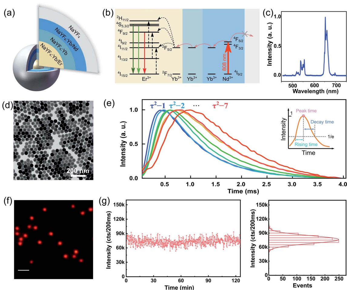
Fig. 2 Photostable uniform nanoprobes with lifetime tunability. (a) Schematic representation of the core–multi-shell \tau^2 -dots using NaYF 4 as host nanocrystals: the core is co-doped by Yb 3+ sensitizer and Er 3+ emitter, the first layer of shell serves as the energy migration layer, doped with 5% Yb 3+ ions, the second shell sensitizes 808 nm photons by 20% Nd 3+ ions with the role of Yb 3+ ions as the secondary sensitizers, and the outer layer of pure NaYF 4 as optically inert shell passivates each single nanoparticle from surface quenchers. (b) Energy level diagrams of the core–multi-shell \tau^2 -dots. (c) The typical upconversion emission spectrum of \tau^2 -dots. (d) TEM characterization of the typical morphology of uniform nanocrystals (Yb 3+ –Nd 3+ –Er 3+ core–multi shell nanoparticles) with an average size of 59 nm. An arbitrary batch ( \tau^2 -5) of \tau^2 -dot used here was chosen from a library of core–multi-shell nanoparticles. (e) The experimentally averaged lifetime curves of \tau^2 -x dots (x = 1, 2, ..., 7) from 20 single dots for each type. (f) Widefield microscopic imaging of \tau^2 -2 under 808 nm excitation. Scale bar: 2 \mu m. (g) Photostability of a single dot under 808 nm excitation in widefield microscopy (the intensity is the sum of covered pixels by a single dot).
