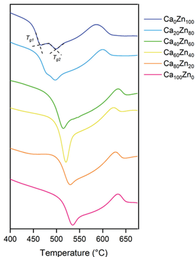
Fig. 4 Differential thermal analysis traces for the \text{Ca}_x\text{Zn}_y lithium alkali-borosilicate glass series, focussing on the glass transition range. The acquisition of T_g (°C) from linear extrapolation of the tangent points for \text{Ca}_0\text{Zn}_{100} is illustrated.
