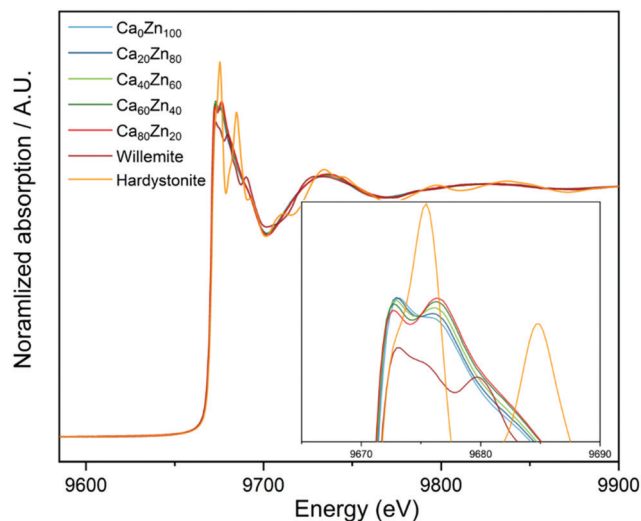
Fig. 1 XANES spectra for the Ca x Zn y glass series, compared with the Zn standards willemite (Zn 2 SiO 4 ) and hardystonite (Ca 2 ZnSi 2 O 7 ).
