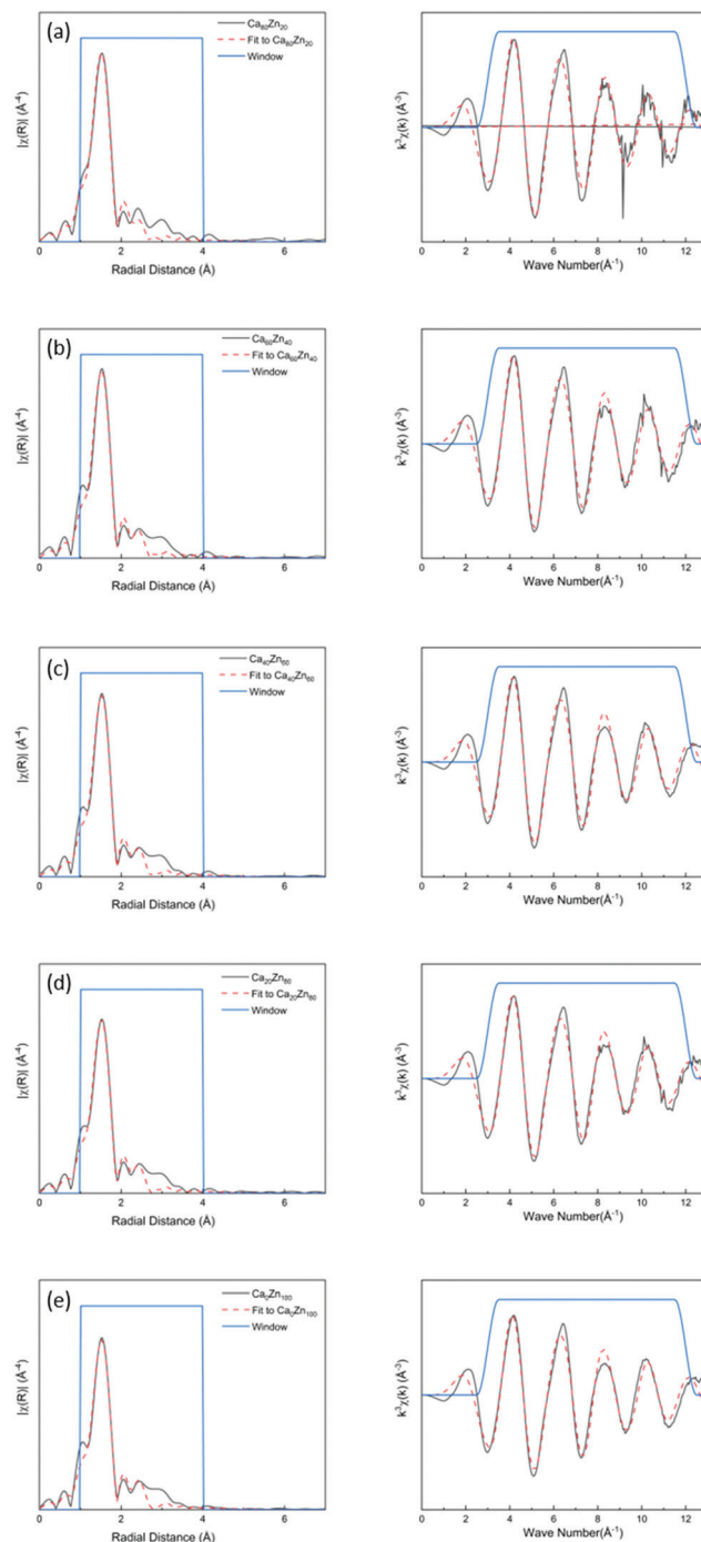
Fig. 2 Extended X-ray Absorption Fine Structure (EXAFS) spectra in radial space and the corresponding k 3 -weighted EXAFS for the Ca x Zn y glass series, for: (a) Ca 80 Zn 20 , (b) Ca 60 Zn 40 , (c) Ca 40 Zn 60 , (d) Ca 20 Zn 80 and (e) Ca 0 Zn 100 .
