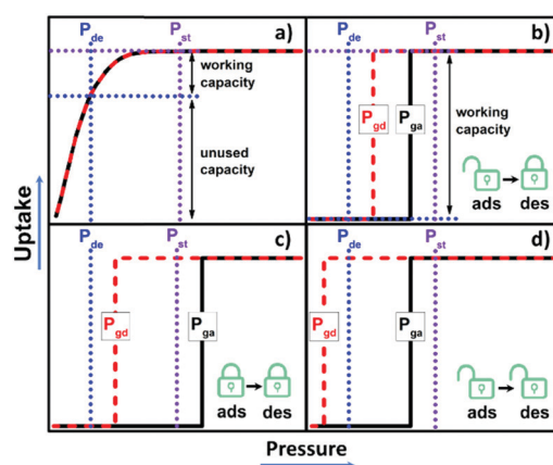
Scheme 1 Comparison of different types of gas sorption isotherms. (a) type I; (b) type F-IV ( P_{de} < P_{gd} < P_{ga} < P_{st} ); (c) type F-IV ( P_{de} < P_{st} < P_{ga} ) and (d) type F-IV ( P_{gd} < P_{de} < P_{ga} < P_{st} ). Black solid line: adsorption; red dash line: desorption; P_{ga} : gate adsorption pressure; P_{gd} : gate desorption pressure; P_{de} : delivery pressure; P_{st} : storage pressure; ads: adsorption; des: desorption.
