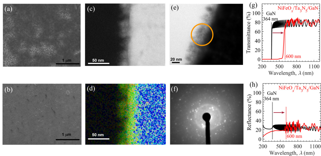
Fig. 2 Modification of \text{Ta}_3\text{N}_5 surface with \text{NiFeO}_x electrocatalyst. Top-view SEM images of \text{NiFeO}_x/\text{Ta}_3\text{N}_5/\text{GaN}/\text{Al}_2\text{O}_3 samples prepared by (a) drop-casting and (b) spin-coating methods. (c) Cross-sectional ADF-STEM image, (d) EDS map, (e) HRTEM image, (f) SAED pattern (corresponding to orange circle in panel (e)), UV-Vis-NIR (g) transmission, and (h) reflectance spectrum with wavelength of \text{NiFeO}_x/\text{Ta}_3\text{N}_5/\text{GaN}/\text{Al}_2\text{O}_3 photoanode developed by spin-coating method (red) and \text{GaN}/\text{Al}_2\text{O}_3 substrate. In panel (d), Fe, Ni, O, N, and Ta elements (with respect to panel (c)) are mapped by green, yellow, orange, light blue, and dark blue colors, respectively.
