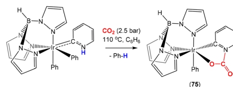
Scheme 19 In situ generation of the Ir-pyridylidene complex and its reactivity towards \text{CO}_2 fixation via 2-atom bridge type 2 activation.
