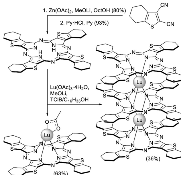
Scheme 27 Synthesis of lutetium(III) complexes with substituted tetrathieno[2,3- b ] porphyrazine. 147
